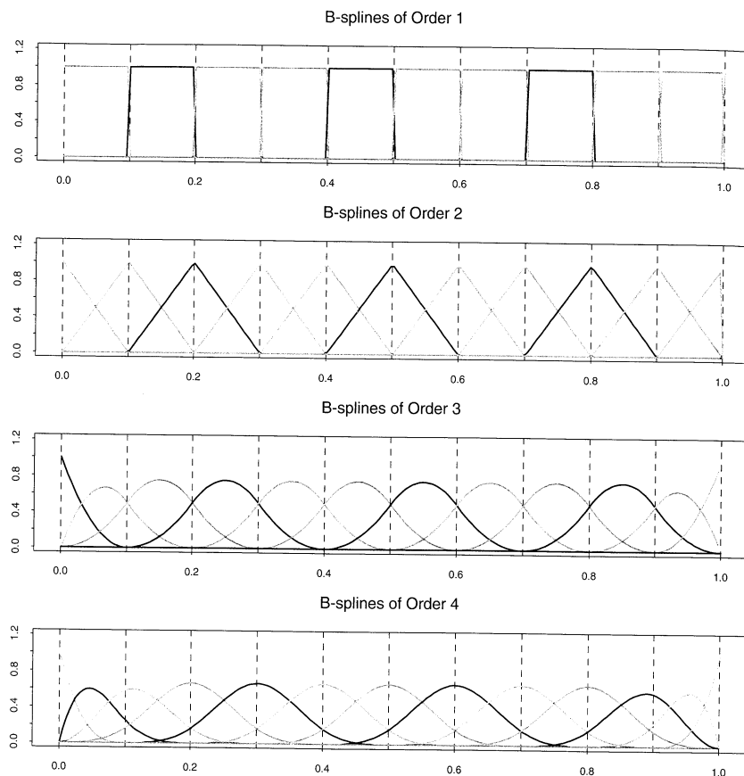
FIGURE 5.17. The sequence of B-splines up to order four with ten knots evenly spaced from 0 to 1. The B-splines have local support; they are nonzero on an interval spanned by M + 1 knots.
