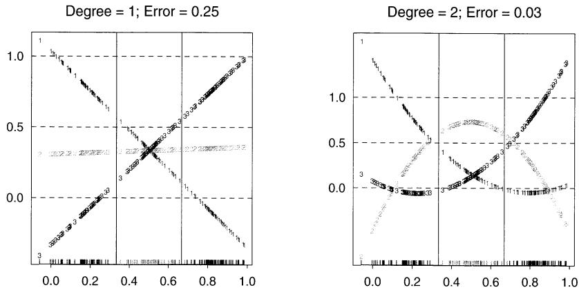
FIGURE 4.3. The effects of masking on linear regression in \mathbb{R} for a three-class problem. The rug plot at the base indicates the positions and class membership of each observation. The three curves in each panel are the fitted regressions to the three-class indicator variables; for example, for the red class, y_{red} is 1 for the red observations, and 0 for the green and blue. The fits are linear and quadratic polynomials. Above each plot is the training error rate. The Bayes error rate is 0.025 for this problem, as is the LDA error rate.
