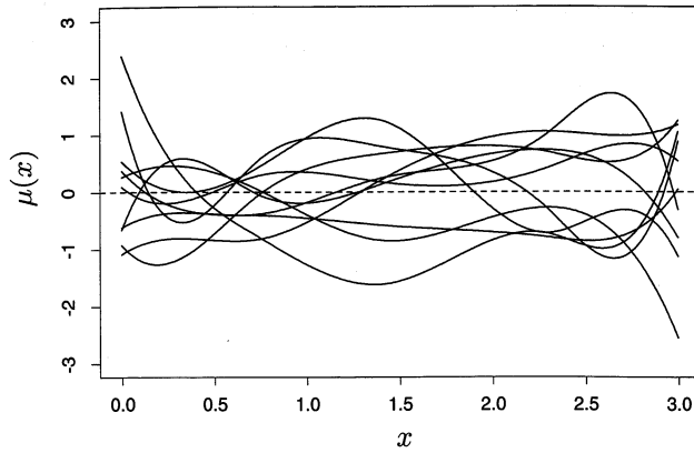
FIGURE 8.3. Smoothing example: Ten draws from the Gaussian prior distribution for the function \mu(x) .
