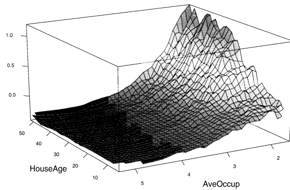
FIGURE 10.16. Partial dependence of house value on median age and average occupancy. There appears to be a strong interaction effect between these two variables.
