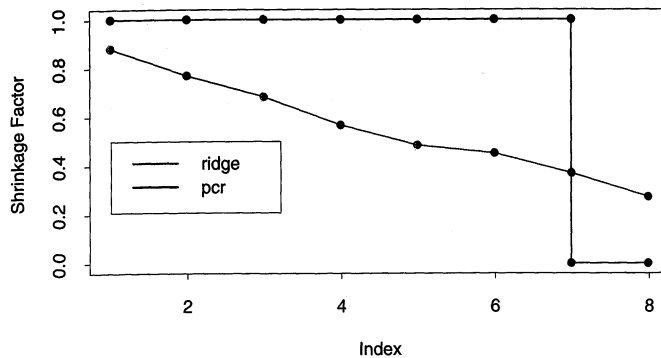
FIGURE 3.10. Ridge regression shrinks the regression coefficients of the principal components, using shrinkage factors d_j^2/(d_j^2 + \lambda) as in (3.47). Principal component regression truncates them. Shown are the shrinkage and truncation patterns corresponding to Figure 3.6, as a function of the principal component index.
