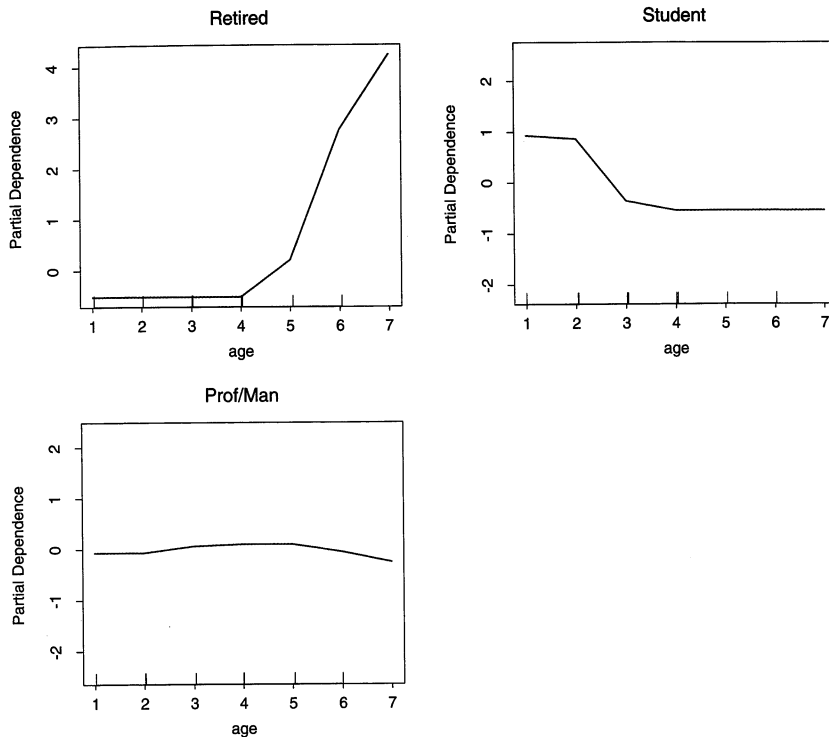
FIGURE 10.21. Partial dependence of the odds of three different occupations on age, for the demographics data.
