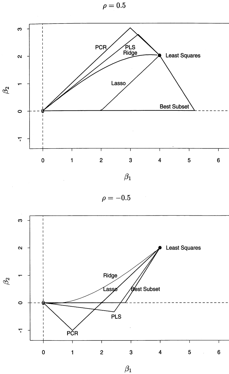
FIGURE 3.11. Coefficient profiles from different methods for a simple problem: two inputs with correlation \pm 0.5 , and the true regression coefficients \beta = (4, 2) .
