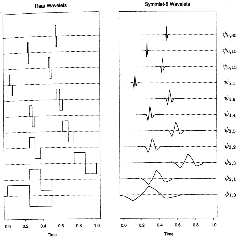
FIGURE 5.13. Some selected wavelets at different translations and dilations for the Haar and symmlet families. The functions have been scaled to suit the display.
