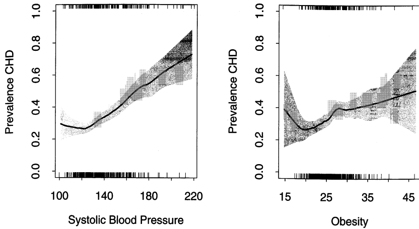
FIGURE 6.12. Each plot shows the binary response CHD (coronary heart disease) as a function of a risk factor for the South African heart disease data. For each plot we have computed the fitted prevalence of CHD using a local linear logistic regression model. The unexpected increase in the prevalence of CHD at the lower ends of the ranges is because these are retrospective data, and some of the subjects had already undergone treatment to reduce their blood pressure and weight. The shaded region in the plot indicates an estimated pointwise standard error band.
