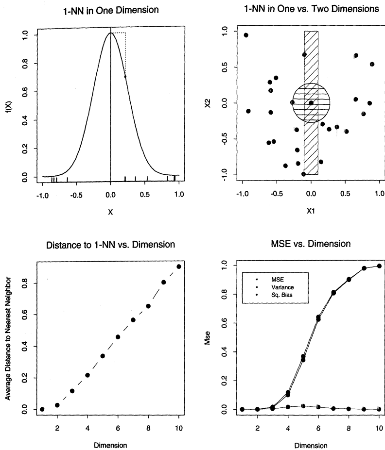
FIGURE 2.7. A simulation example, demonstrating the curse of dimensionality and its effect on MSE, bias and variance. The input features are uniformly distributed in [-1, 1]^p for p = 1, \dots, 10 . The top left panel shows the target function (no noise) in \mathbb{R} : f(X) = e^{-8||X||^2} , and demonstrates the error that 1-nearest neighbor makes in estimating f(0) . The training point is indicated by the blue tick mark. The top right panel illustrates why the radius of the 1-nearest neighborhood increases with dimension p . The lower left panel shows the average radius of the 1-nearest neighborhoods. The lower-right panel shows the MSE, squared bias and variance curves as a function of dimension p .
