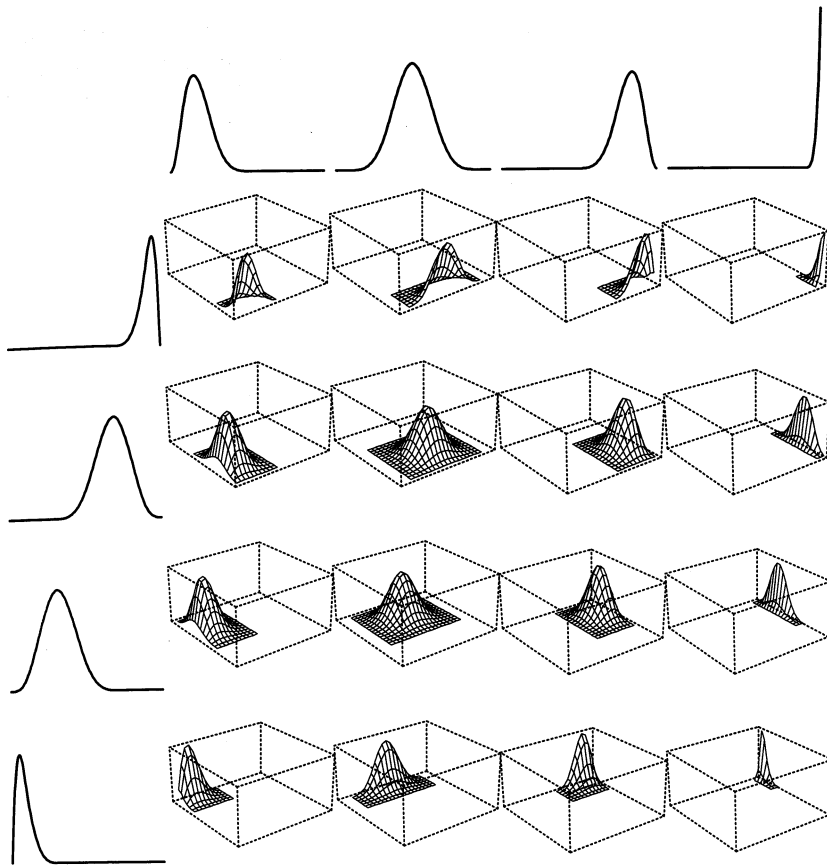
FIGURE 5.10. A tensor product basis of B-splines, showing some selected pairs. Each two-dimensional function is the tensor product of the corresponding one-dimensional marginals.
