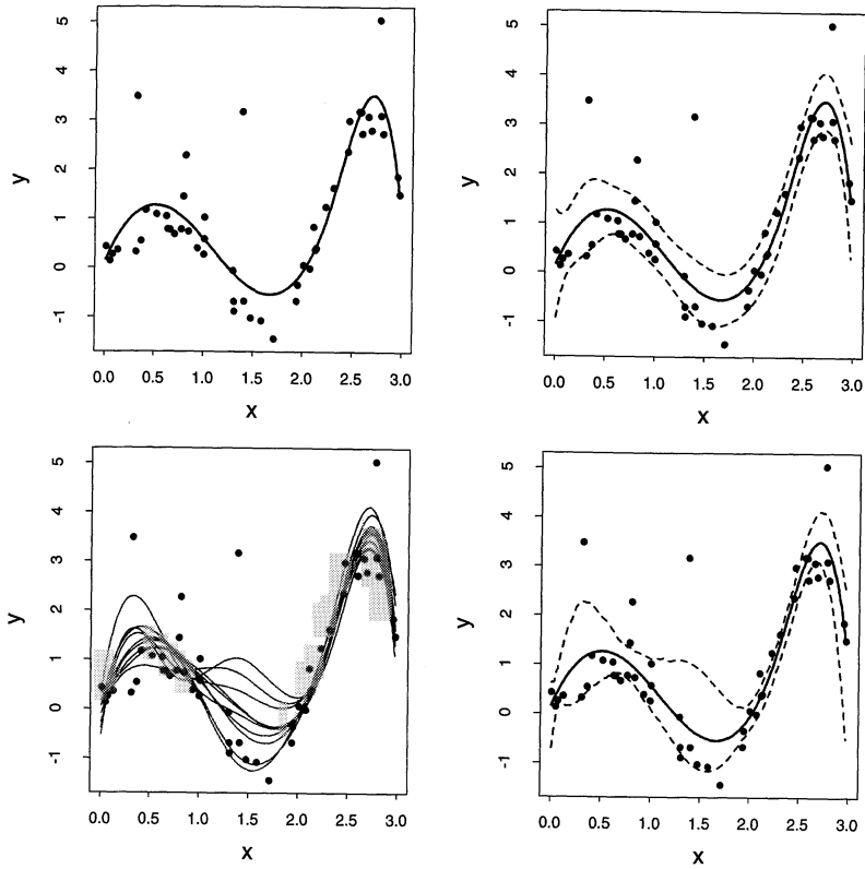
FIGURE 8.2. Top left: B-spline smooth of data. Top right: B-spline smooth plus and minus 1.96 \times standard error bands. Bottom left: ten bootstrap replicates of the B-spline smooth. Bottom right: B-spline smooth with 95% standard error bands computed from the bootstrap distribution.
