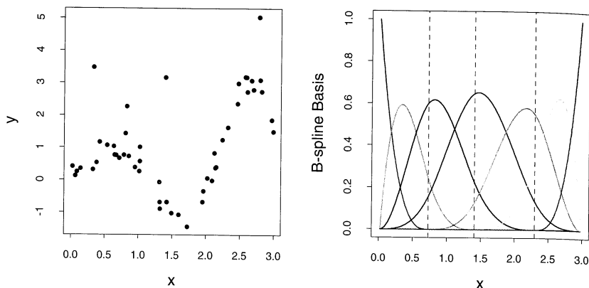
FIGURE 8.1. Left panel: data for smoothing example. Right panel: set of seven B-spline basis functions. The broken vertical lines indicate the placement of the three knots.
