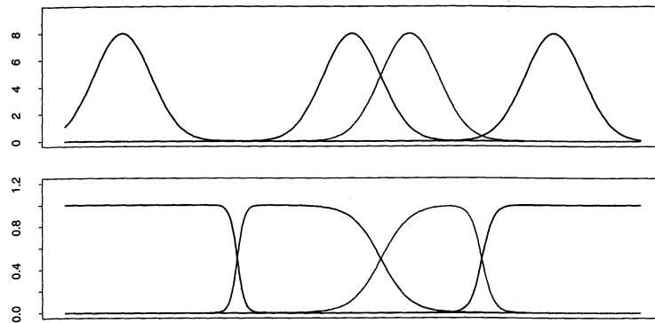
FIGURE 6.16. Gaussian radial basis functions in \mathbb{R} with fixed width can leave holes (top panel). Renormalized Gaussian radial basis functions avoid this problem, and produce basis functions similar in some respects to B-splines.
