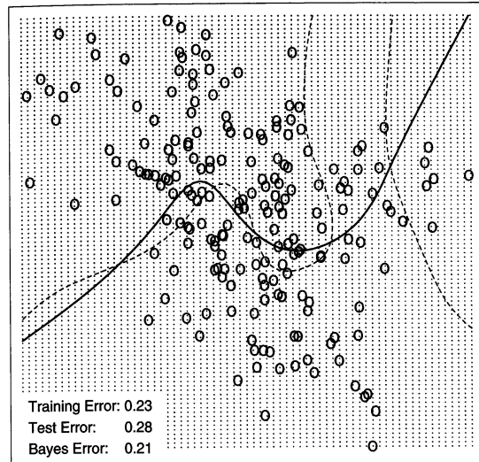
Additive Natural Cubic Splines - 4 df each
