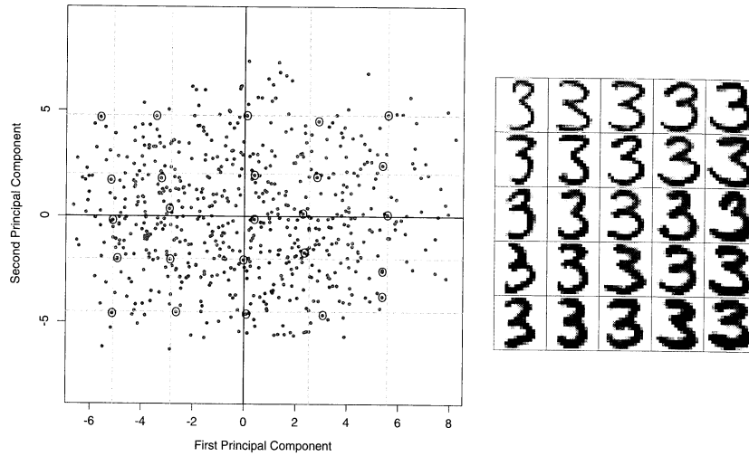
FIGURE 14.23. Left plot: the first two principal components of the handwritten threes. The circled points are the closest projected images to the vertices of a grid, defined by the marginal quantiles of the principal components. Right plot: the images corresponding to the red-circled points. These show the nature of the first two principal components.
