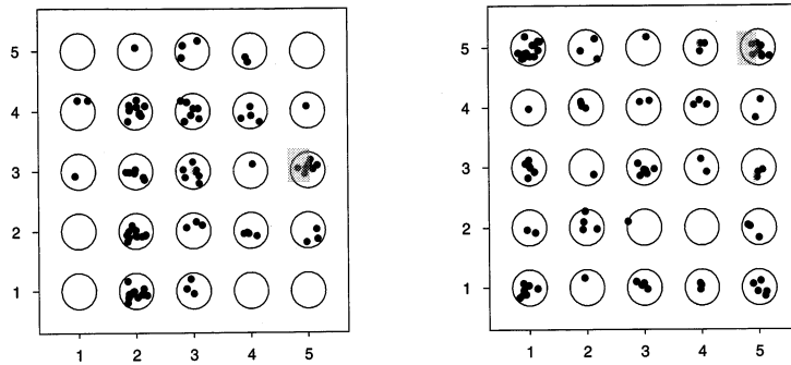
FIGURE 14.16. Self-organizing map applied to half-sphere data example. Left panel is the initial configuration, right panel the final one. The 5 \times 5 grid of prototypes are indicated by circles, and the points that project to each prototype are plotted randomly within the corresponding circle.
