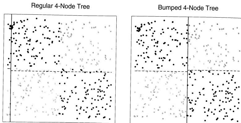
FIGURE 8.12. Data with two features and two classes (green and red), displaying a pure interaction. The left panel shows the partition found by three splits of a standard, greedy, tree-growing algorithm. The vertical blue line near the left edge is the first split, and the broken lines are the two subsequent splits. The algorithm has no idea where to make a good initial split, and makes a poor choice. The right panel shows the near-optimal splits found by bumping the tree-growing algorithm 20 times.
