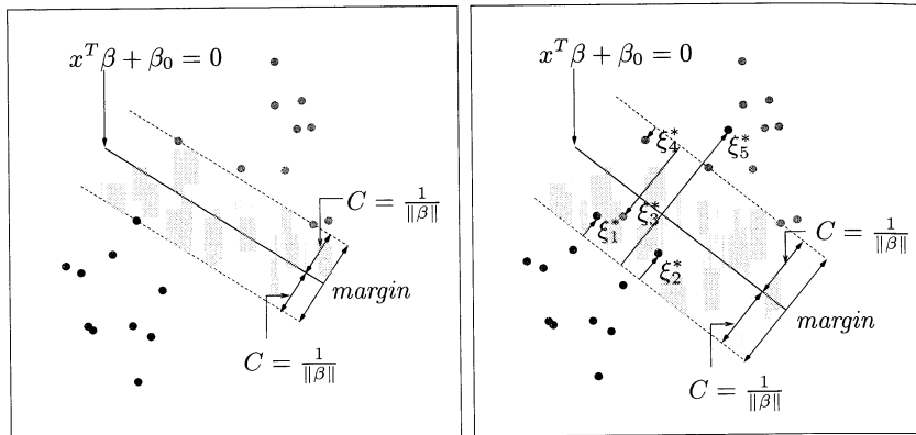
FIGURE 12.1. Support vector classifiers. The left panel shows the separable case. The decision boundary is the solid line, while broken lines bound the shaded maximal margin of width 2C = 2/\|\beta\| . The right panel shows the nonseparable (overlap) case. The points labeled \xi_j^* are on the wrong side of their margin by an amount \xi_j^* = C\xi_j ; points on the correct side have \xi_j^* = 0 . The margin is maximized subject to a total budget \sum \xi_i \leq \text{constant} . Hence \sum \xi_j^* is the total distance of points on the wrong side of their margin.
