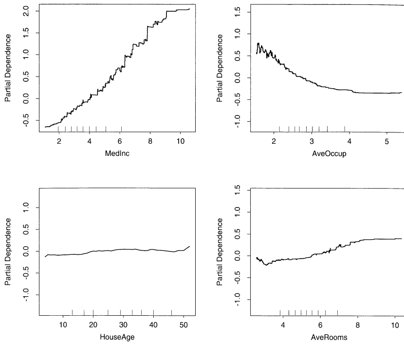
FIGURE 10.15. Partial dependence of housing value on the nonlocation variables for the California housing data.
