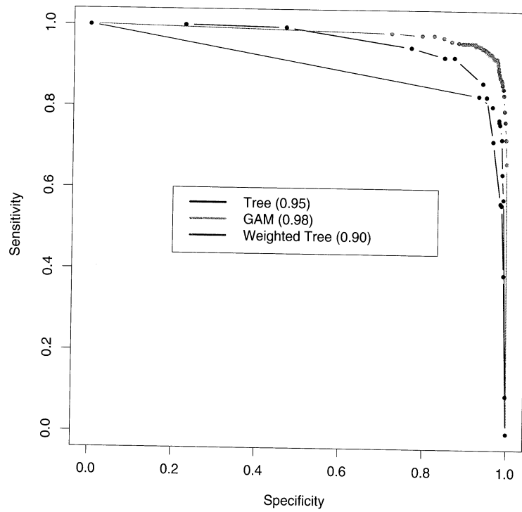
FIGURE 9.6. ROC curves for the classification rules fit to the spam data. Curves that are closer to the northeast corner represent better classifiers. In this case the GAM classifier dominates the trees. The weighted tree achieves better sensitivity for higher specificity than the unweighted tree. The numbers in the legend represent the area under the curve.
