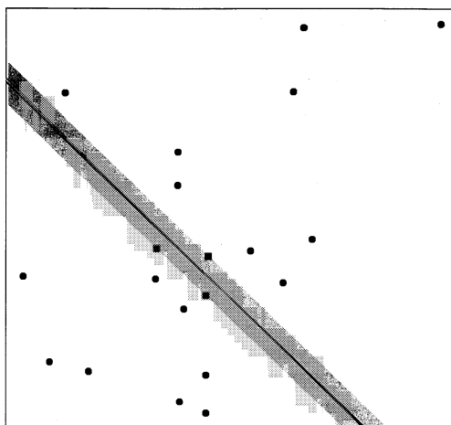
FIGURE 4.15. The same data as in Figure 4.13. The shaded region delineates the maximum margin separating the two classes. There are three support points indicated, which lie on the boundary of the margin, and the optimal separating hyperplane (blue line) bisects the slab. Included in the figure is the boundary found using logistic regression (red line), which is very close to the optimal separating hyperplane (see Section 12.3.3).
