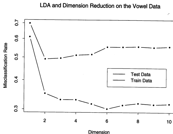
FIGURE 4.10. Training and test error rates for the vowel data, as a function of the dimension of the discriminant subspace. In this case the best error rate is for dimension 2. Figure 4.11 shows the decision boundaries in this space.
