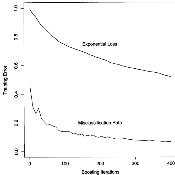
FIGURE 10.3. Simulated data, boosting with stumps: misclassification error rate on the training set, and average exponential loss: (1/N) \sum_{i=1}^N \exp(-y_i f(x_i)) .
