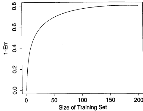
FIGURE 7.8. Hypothetical learning curve for a classifier on a given task; a plot of 1 - \text{Err} versus the size of the training set N . With a dataset of 200 observations, fivefold cross-validation would use training sets of size 160, which would behave much like the full set. However, with a dataset of 50 observations fivefold cross-validation would use training sets of size 40, and this would result in a considerable overestimate of prediction error.
