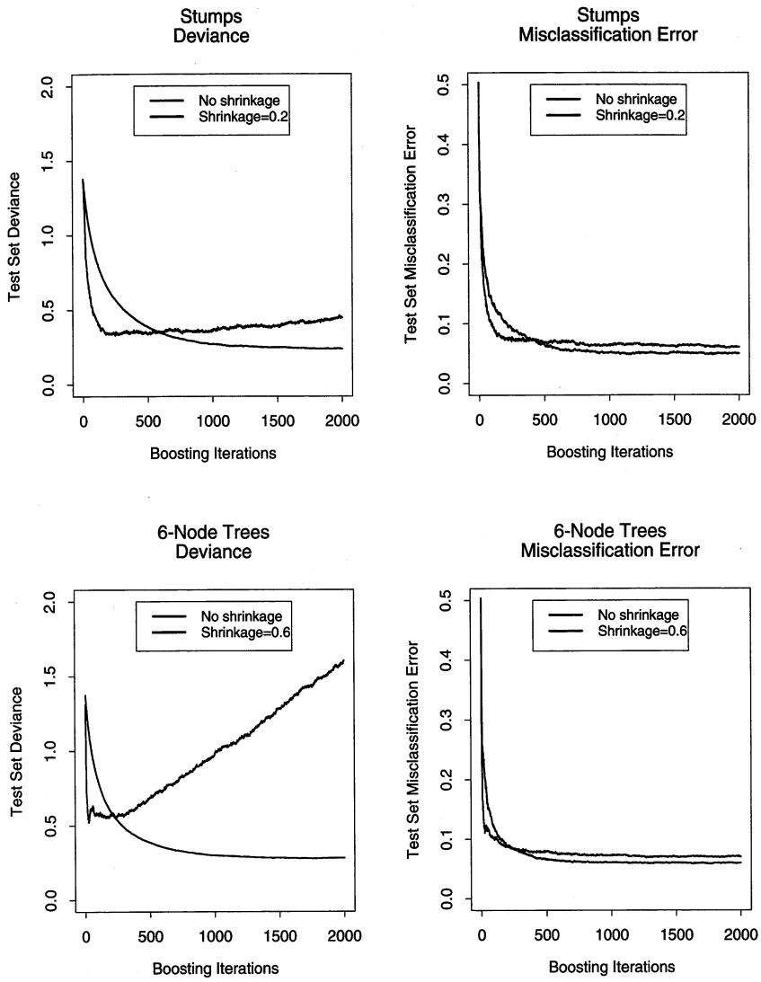
FIGURE 10.11. Test error curves for simulated example (10.2) of Figure 10.9, using MART. The models were trained using binomial deviance, either stumps or six terminal-node trees, and with or without shrinkage. The left panels report test deviance, while the right panels show misclassification error. The beneficial effect of shrinkage can be seen in all cases, especially for deviance in the left panels.
