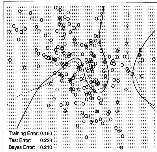
Neural Network - 10 Units, Weight Decay=0.02
