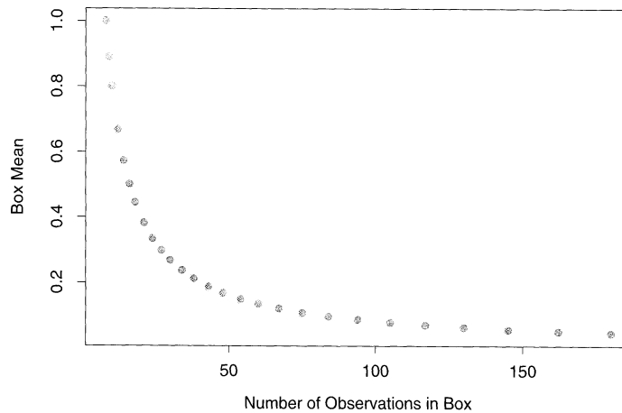
FIGURE 9.8. Box mean as a function of number of observations in the box.
