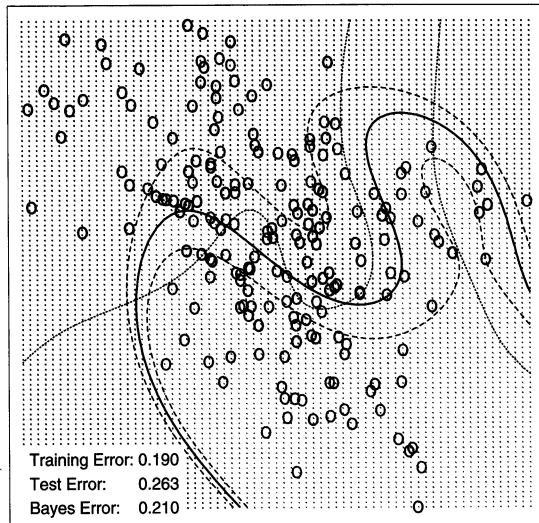
LR - Radial Kernel in Feature Space
