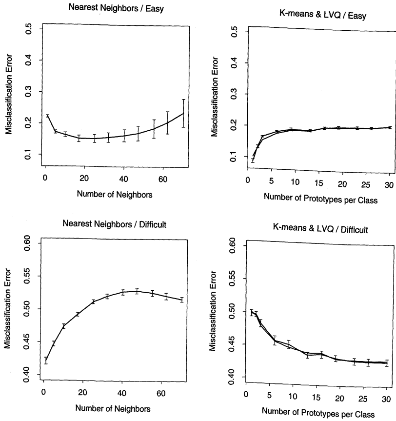
FIGURE 13.5. Mean \pm one standard error of misclassification error for nearest-neighbors, K -means (blue) and LVQ (red) over ten realizations for two simulated problems: “easy” and “difficult,” described in the text.
