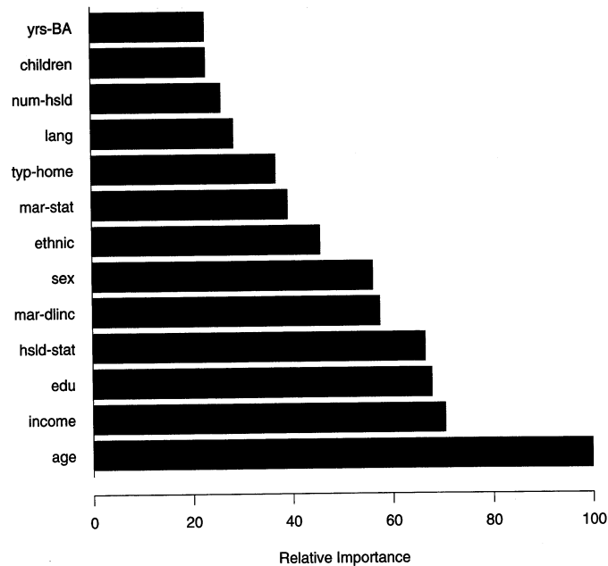
FIGURE 10.19. Relative importance of the predictors as averaged over all classes for the demographics data.
