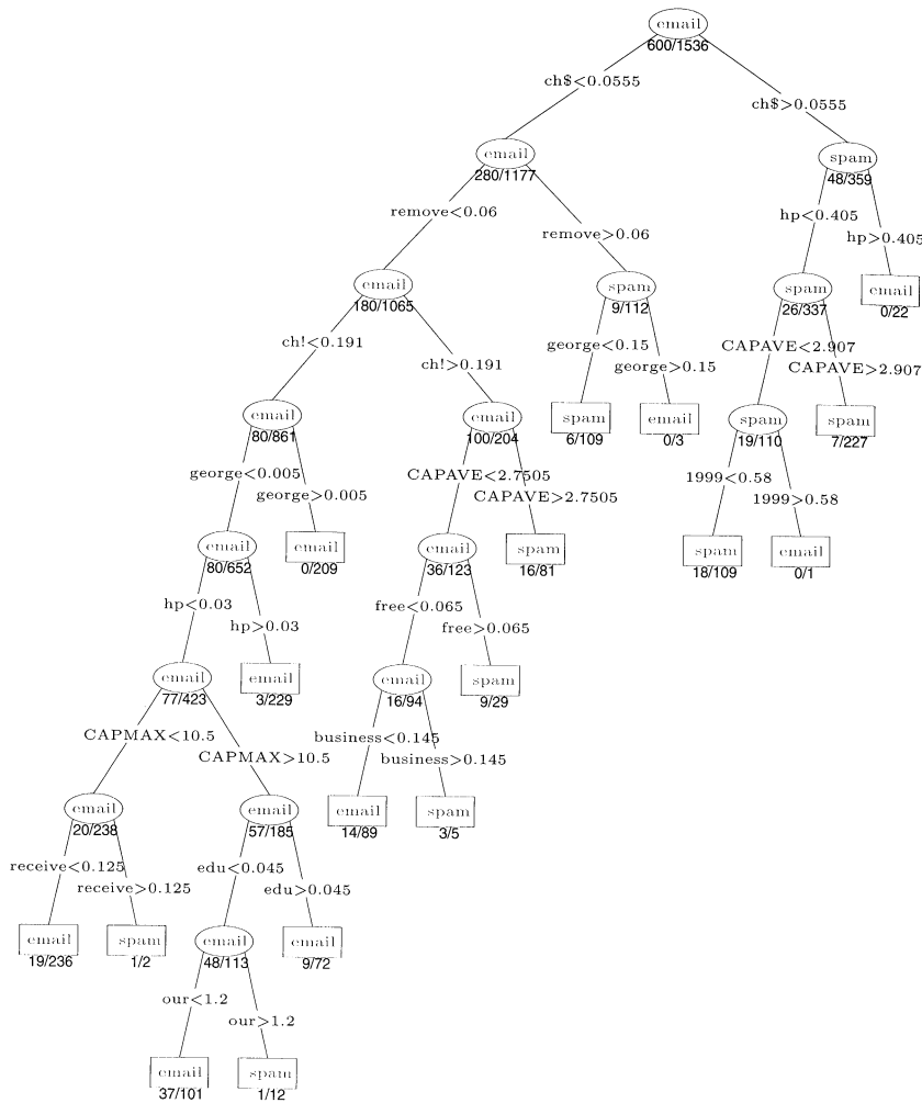
FIGURE 9.5. The pruned tree for the spam example. The split variables are shown in blue on the branches, and the classification is shown in every node. The numbers under the terminal nodes indicate misclassification rates on the test data.
