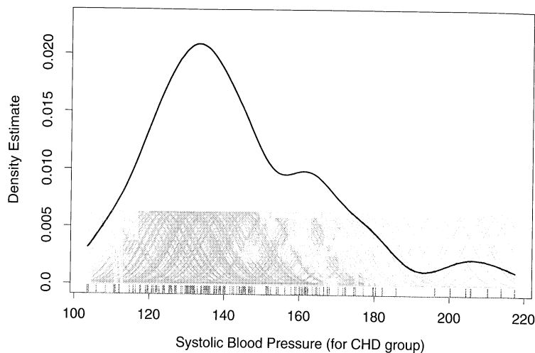
FIGURE 6.13. A kernel density estimate for systolic blood pressure (for the CHD group). The density estimate at each point is the average contribution from each of the kernels at that point. We have scaled the kernels down by a factor of 10 to make the graph readable.
