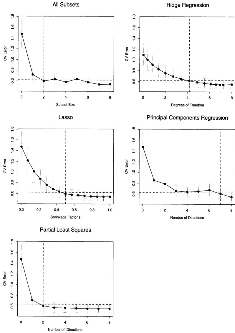
FIGURE 3.6. Estimated prediction error curves and their standard errors for the various selection and shrinkage methods. Each curve is plotted as a function of the corresponding complexity parameter for that method. The horizontal axis has been chosen so that the model complexity increases as we move from left to right. The prediction error estimates and their standard errors were obtained by tenfold cross-validation; full details are given in Section 7.10. The least complex model within one standard error of the best is chosen.
