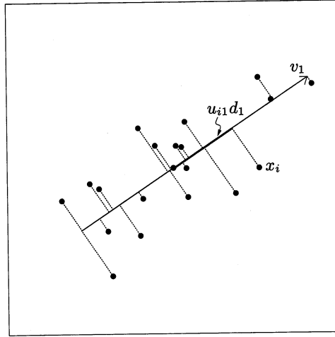
FIGURE 14.20. The first linear principal component of a set of data. The line minimizes the total squared distance from each point to its orthogonal projection onto the line.
