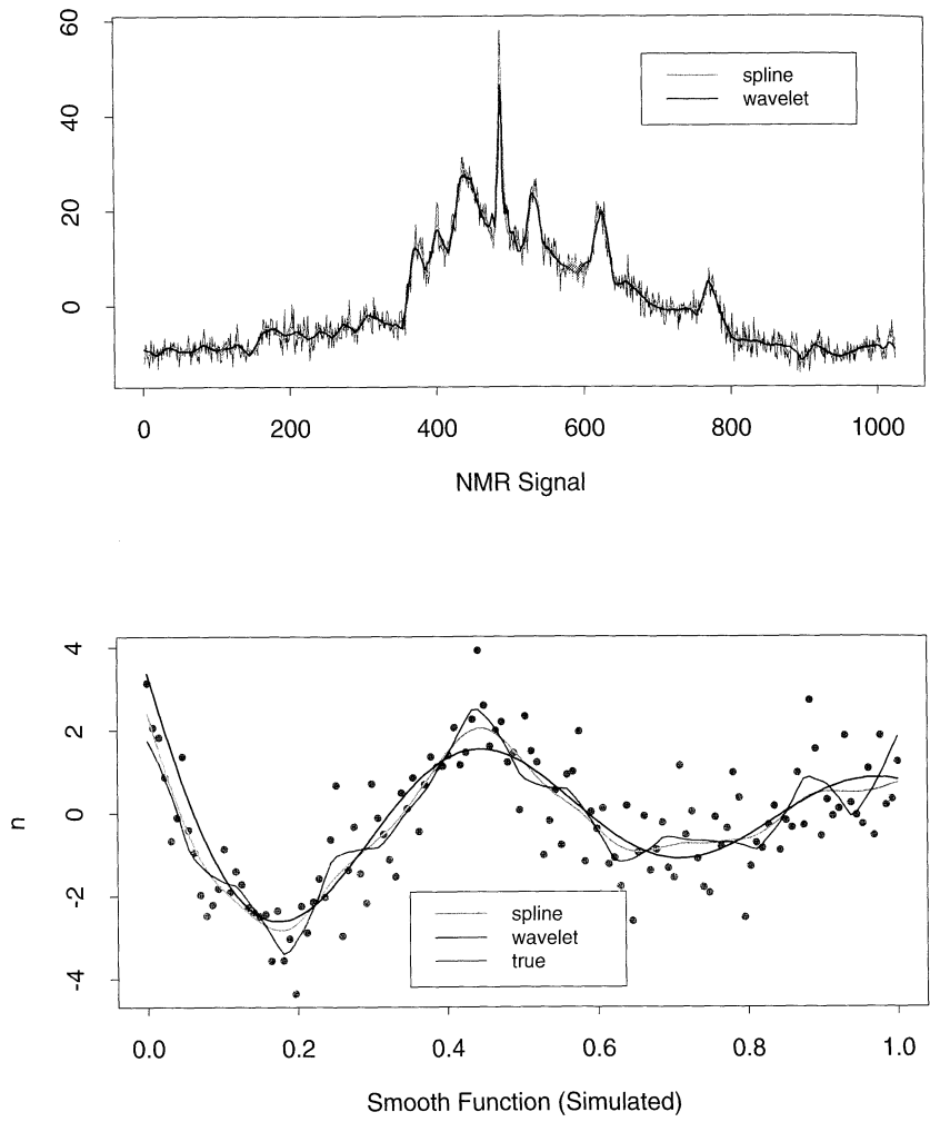
FIGURE 5.16. Wavelet smoothing compared with smoothing splines on two examples. Each panel compares the SURE-shrunk wavelet fit to the cross-validated smoothing spline fit.
