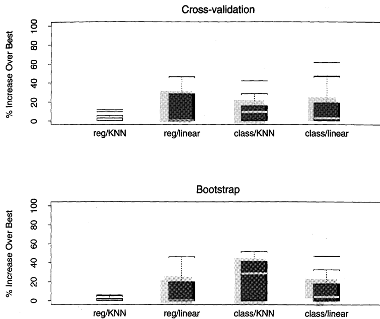
FIGURE 7.11. Boxplots show the distribution of the relative error 100 \cdot [\text{Err}_{\hat{\alpha}} - \min_{\alpha} \text{Err}(\alpha)] / [\max_{\alpha} \text{Err}(\alpha) - \min_{\alpha} \text{Err}(\alpha)] over the four scenarios of Figure 7.3. This is the error in using the chosen model relative to the best model. There are 20 training sets represented in each boxplot.
