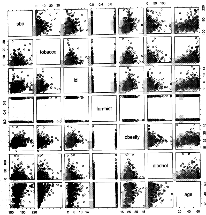
FIGURE 4.12. A scatterplot matrix of the South African heart disease data. Each plot shows a pair of risk factors, and the cases and controls are color coded (red is a case). The variable family history of heart disease (famhist) is binary (yes or no).
