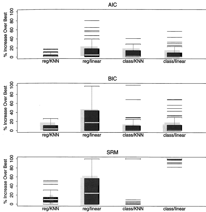
FIGURE 7.7. Boxplots show the distribution of the relative error 100 \times [\text{Err}(\hat{\alpha}) - \min_{\alpha} \text{Err}(\alpha)] / [\max_{\alpha} \text{Err}(\alpha) - \min_{\alpha} \text{Err}(\alpha)] over the four scenarios of Figure 7.3. This is the error in using the chosen model relative to the best model. There are 100 training sets each of size 50 represented in each boxplot, with the errors computed on test sets of size 500.
