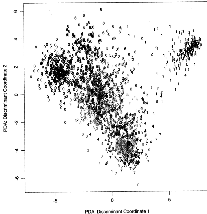
FIGURE 12.10. The first two penalized canonical variates, evaluated for the test data. The circles indicate the class centroids. The first coordinate contrasts mainly 0's and 1's, while the second contrasts 6's and 7/9's.
