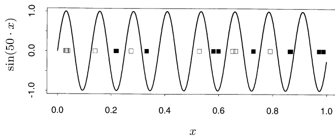
FIGURE 7.5. The solid curve is the function \sin(50x) for x \in [0, 1] . The blue (solid) and green (hollow) points illustrate how the associated indicator function I(\sin(\alpha x) > 0) can shatter (separate) an arbitrarily large number of points by choosing an appropriately high frequency \alpha .
