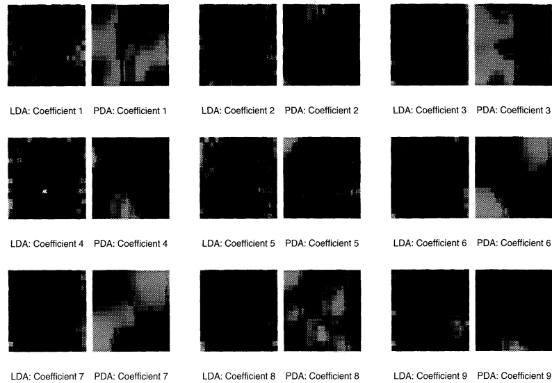
FIGURE 12.9. The images appear in pairs, and represent the nine discriminant coefficient functions for the digit recognition problem. The left member of each pair is the LDA coefficient, while the right member is the PDA coefficient, regularized to enforce spatial smoothness.
