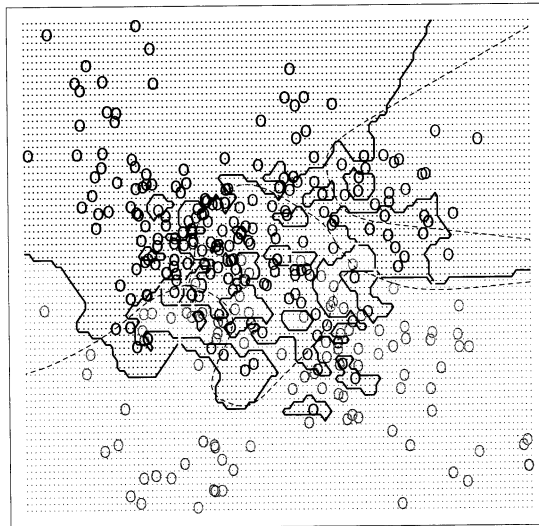
1-Nearest Neighbor
