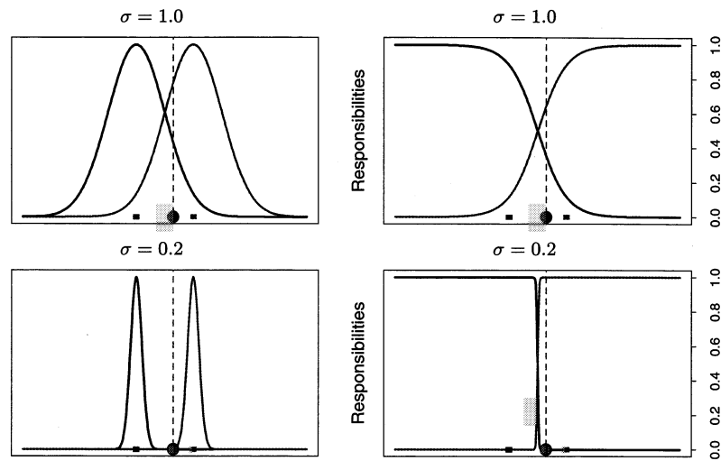
FIGURE 14.7. Left panels: two Gaussian densities g_0(x) and g_1(x) (blue and orange) on the real line, and a single data point (green dot) at x = 0.5 . The colored squares are plotted at x = -1.0 and x = 1.0 , the means of each density. Right panels: the relative densities g_0(x)/(g_0(x)+g_1(x)) and g_1(x)/(g_0(x)+g_1(x)) , called the “responsibilities” of each cluster, for this data point. In the top panels, the Gaussian standard deviation \sigma = 1.0 ; in the bottom panels \sigma = 0.2 . The EM algorithm uses these responsibilities to make a “soft” assignment of each data point to each of the two clusters. When \sigma is fairly large, the responsibilities can be near 0.5 (they are 0.36 and 0.64 in the top right panel). As \sigma \rightarrow 0 , the responsibilities \rightarrow 1 , for the cluster center closest to the target point, and 0 for all other clusters. This “hard” assignment is seen in the bottom right panel.
