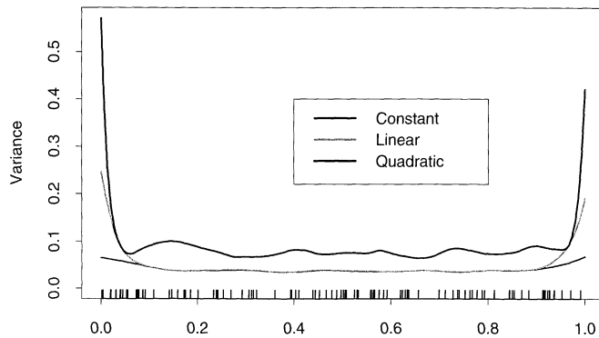
FIGURE 6.6. The variances functions ||l(x)||^2 for local constant, linear and quadratic regression, for a metric bandwidth ( \lambda = 0.2 ) tri-cube kernel.
