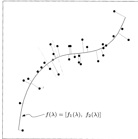
FIGURE 14.25. The principal curve of a set of data. Each point on the curve is the average of all data points that project there.
