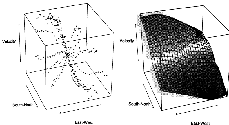
FIGURE 6.8. The left panel shows three-dimensional data, where the response is the velocity measurements on a galaxy, and the two predictors record positions on the celestial sphere. The unusual “star” shaped design indicates the way the measurements were made, and results in an extremely irregular boundary. The right panel shows the results of local linear regression smoothing in \mathbb{R}^2 , using a nearest-neighbor window with 15% of the data.
