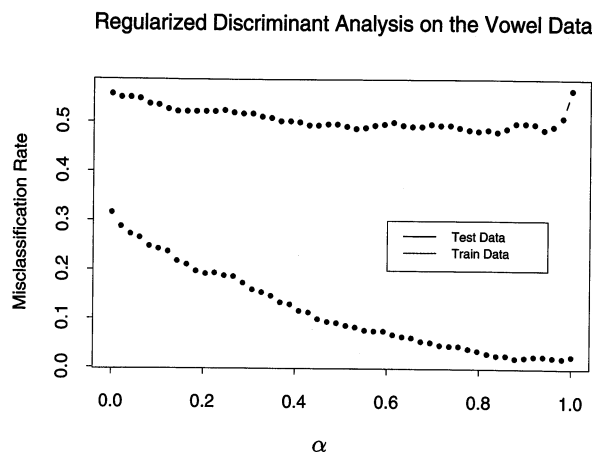
FIGURE 4.7. Test and training errors for the vowel data, using regularized discriminant analysis with a series of values of \alpha \in [0, 1] . The optimum for the test data occurs around \alpha = 0.9 , close to quadratic discriminant analysis.
