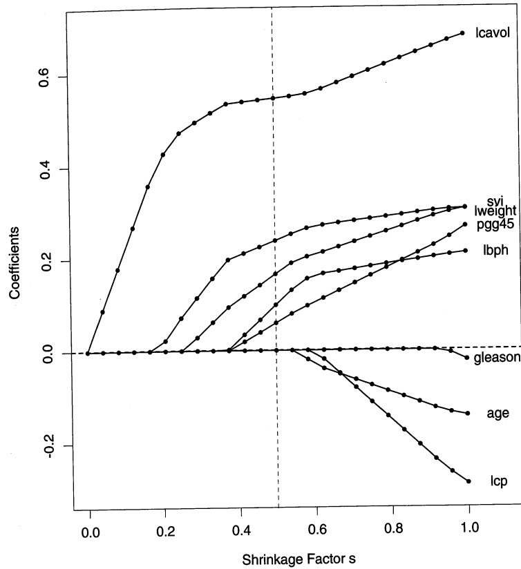
FIGURE 3.9. Profiles of lasso coefficients, as tuning parameter t is varied. Coefficients are plotted versus s = t / \sum_1^p |\hat{\beta}_j| . A vertical line is drawn at s = 0.5 , the value chosen by cross-validation. Compare Figure 3.7 on page 61; the lasso profiles hit zero, while those for ridge do not.
