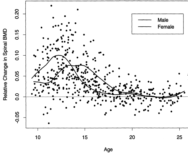
FIGURE 5.6. The response is the relative change in bone mineral density measured at the spine in adolescents, as a function of age. A separate smoothing spline was fit to the males and females, with \lambda \approx 0.00022 . This choice corresponds to about 12 degrees of freedom.
