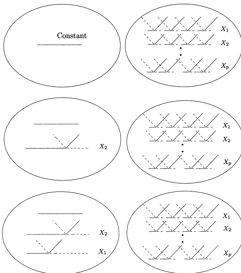
FIGURE 9.10. Schematic of the MARS forward model-building procedure. On the left are the basis functions currently in the model: initially, this is the constant function h(X) = 1 . On the right are all candidate basis functions to be considered in building the model. These are pairs of piecewise linear basis functions as in Figure 9.9, with knots t at all unique observed values x_{ij} of each predictor X_j . At each stage we consider all products of a candidate pair with a basis function in the model. The product that decreases the residual error the most is added into the current model. Above we illustrate the first three steps of the procedure, with the selected functions shown in red.
