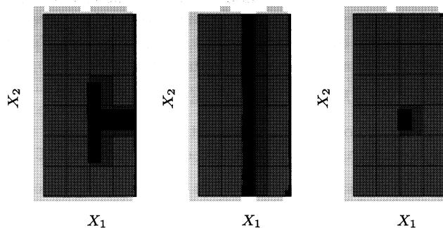
FIGURE 14.1. Simplifications for association rules. Here there are two inputs X_1 and X_2 , taking four and six distinct values, respectively. The red squares indicate areas of high density. To simplify the computations, we assume that the derived subset corresponds to either a single value of an input or all values. With this assumption we could find either the middle or right pattern, but not the left one.
