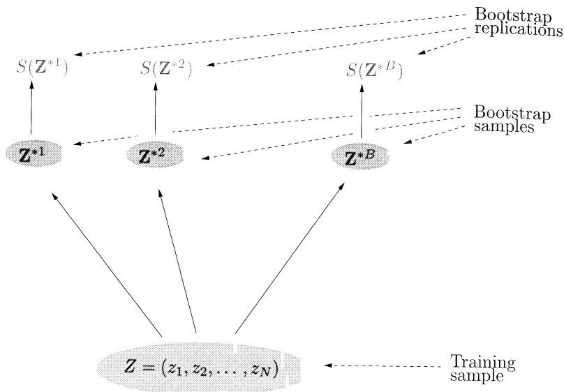
FIGURE 7.10. Schematic of the bootstrap process. We wish to assess the statistical accuracy of a quantity S(\mathbf{Z}) computed from our dataset. B training sets \mathbf{Z}^{*b} , b = 1, \dots, B each of size N are drawn with replacement from the original dataset. The quantity of interest S(\mathbf{Z}) is computed from each bootstrap training set, and the values S(\mathbf{Z}^{*1}), \dots, S(\mathbf{Z}^{*B}) are used to assess the statistical accuracy of S(\mathbf{Z}) .
