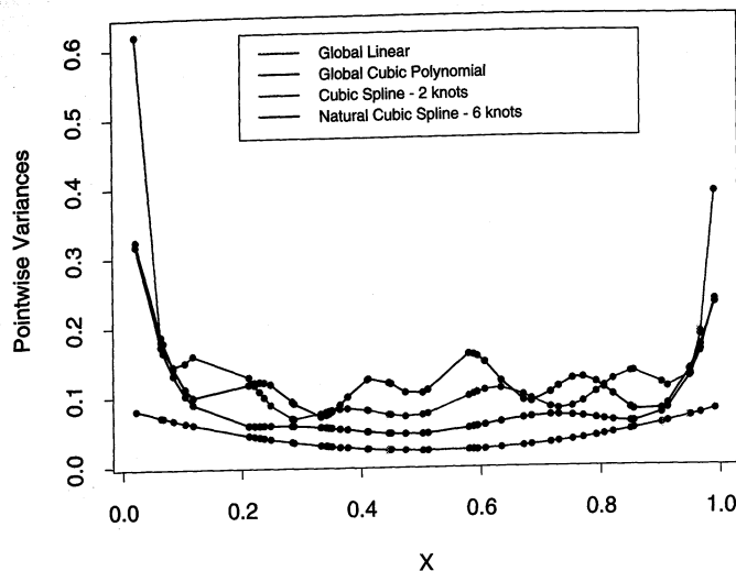
FIGURE 5.3. Pointwise variance curves for four different models, with X consisting of 50 points drawn at random from U[0, 1] , and an assumed error model with constant variance. The linear and cubic polynomial fits have two and four degrees of freedom respectively, while the cubic spline and natural cubic spline each have six degrees of freedom. The cubic spline has two knots at 0.33 and 0.66, while the natural spline has boundary knots at 0.1 and 0.9, and four interior knots uniformly spaced between them.
