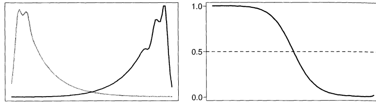
FIGURE 6.15. The population class densities may have interesting structure (left) that disappears when the posterior probabilities are formed (right).
