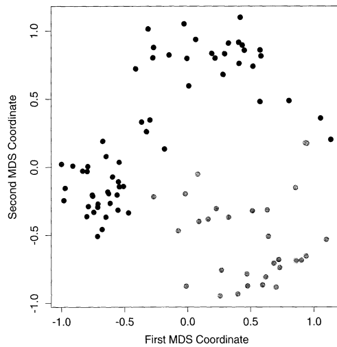
FIGURE 14.32. First two coordinates for half-sphere data, from classical multidimensional scaling.
