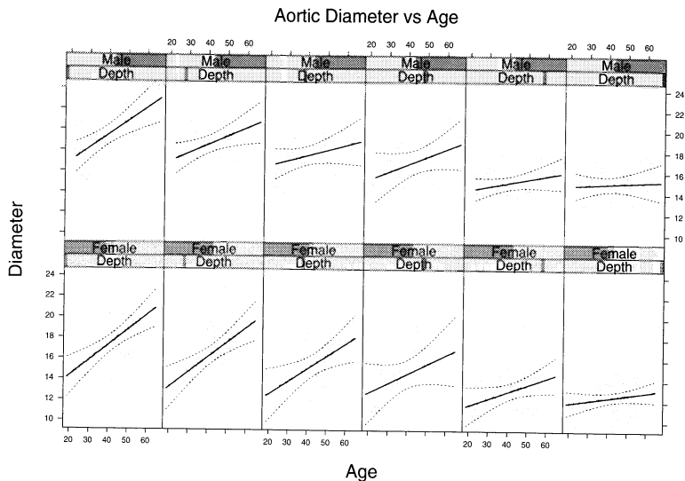
FIGURE 6.10. In each panel the aorta diameter is modeled as a linear function of age. The coefficients of this model vary with gender and depth down the aorta (left is near the top, right is low down). There is a clear trend in the coefficients of the linear model.
