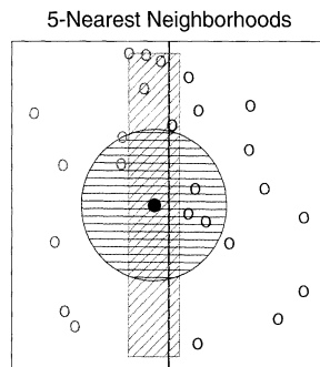
FIGURE 13.13. The points are uniform in the cube, with the vertical line separating class red and green. The vertical strip denotes the 5-nearest-neighbor region using only the horizontal coordinate to find the nearest-neighbors for the target point (solid dot). The sphere shows the 5-nearest-neighbor region using both coordinates, and we see in this case it has extended into the class-red region (and is dominated by the wrong class in this instance).
