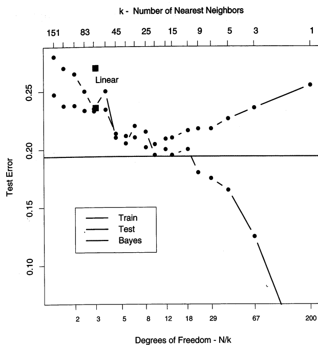
FIGURE 2.4. Misclassification curves for the simulation example used in Figures 2.1, 2.2 and 2.3. A single training sample of size 200 was used, and a test sample of size 10,000. The red curves are test and the green are training error for k -nearest-neighbor classification. The results for linear regression are the bigger green and red squares at three degrees of freedom. The purple line is the optimal Bayes Error Rate.
