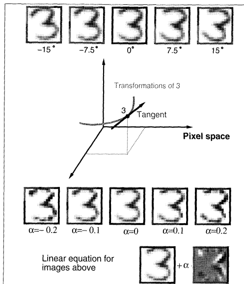
FIGURE 13.10. The top row shows a “3” in its original orientation (middle) and rotated versions of it. The green curve in the middle of the figure depicts this set of rotated “3” in 256-dimensional space. The red line is the tangent line to the curve at the original image, with some “3”s on this tangent line, and its equation shown at the bottom of the figure.
