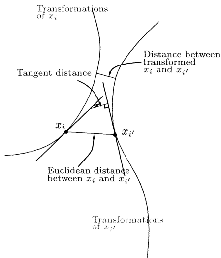
FIGURE 13.11. Tangent distance computation for two images x_i and x_{i'} . Rather than using the Euclidean distance between x_i and x_{i'} , or the shortest distance between the two curves, we use the shortest distance between the two tangent lines.
