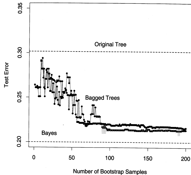
FIGURE 8.10. Error curves for the bagging example of Figure 8.9. Shown is the test error of the original tree and bagged trees as a function of the number of bootstrap samples. The green points correspond to majority vote, while the purple points average the probabilities.
