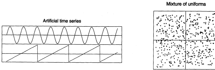
FIGURE 14.31. Projection-pursuit solutions to the artificial time series problem of Figure 14.27 (left panel), and the mixture of uniforms problem of Figure 14.28 (right panel). These solutions were obtained using the generalized logistic regression model (14.67).
