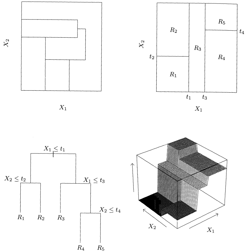
FIGURE 9.2. Partitions and CART. Top right panel shows a partition of a two-dimensional feature space by recursive binary splitting, as used in CART, applied to some fake data. Top left panel shows a general partition that cannot be obtained from recursive binary splitting. Bottom left panel shows the tree corresponding to the partition in the top right panel, and a perspective plot of the prediction surface appears in the bottom right panel.
