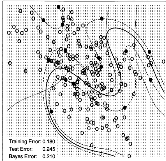
SVM - Radial Kernel in Feature Space
