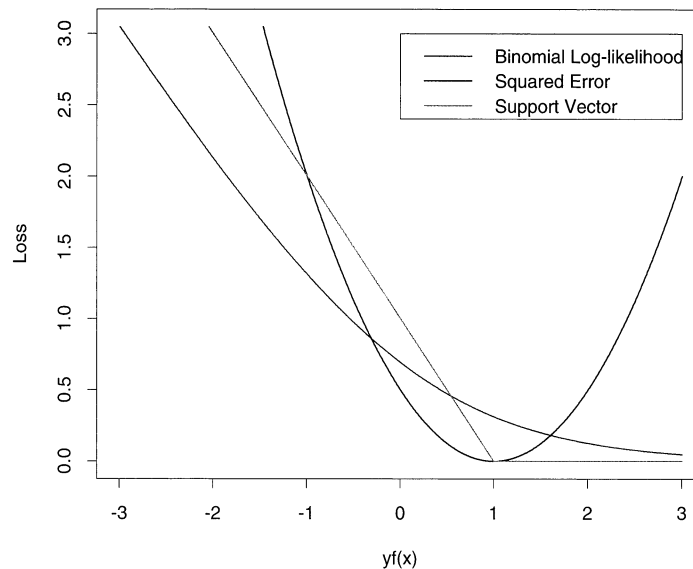
FIGURE 12.4. The support vector loss function, compared to the (negative) log-likelihood loss for logistic regression, and squared-error loss. All are shown as a function of yf rather than f , because of the symmetry in all three between the y = +1 and y = -1 case. The log-likelihood has the same asymptotes as the SVM loss, but is rounded in the interior.
