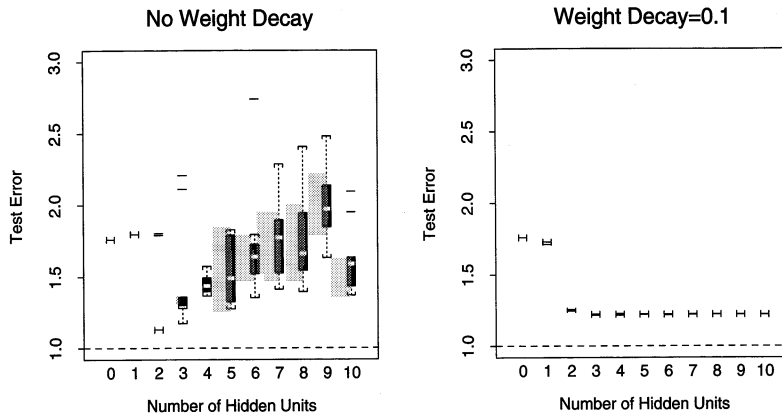
FIGURE 11.7. Boxplots of test error, for simulated data example, relative to the Bayes error. True function is a sum of two sigmoids. The test error is displayed for ten different starting weights, for a single hidden layer neural network with the number units as indicated. The two panels represent no weight decay (left) and strong weight decay \lambda = 0.1 (right).
