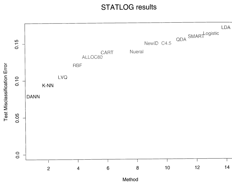
FIGURE 13.8. Test-error performance for a number of classifiers, as reported by the STATLOG project. The entry DANN is a variant of k -nearest neighbors, using an adaptive metric (Section 13.4.2).
