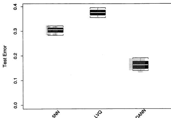
FIGURE 13.15. Ten-dimensional simulated example: boxplots of the test error rates over ten realizations, for standard 5-nearest-neighbors, LVQ with 50 centers, and discriminant-adaptive 5-nearest-neighbors
