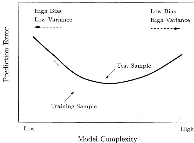
FIGURE 7.1. Behavior of test sample and training sample error as the model complexity is varied.
