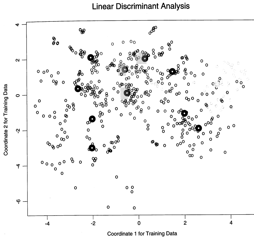
FIGURE 4.4. A two-dimensional plot of the vowel training data. There are eleven classes with X \in \mathbb{R}^{10} , and this is the best view in terms of a LDA model (Section 4.3.3). The heavy circles are the projected mean vectors for each class. The class overlap is considerable.
