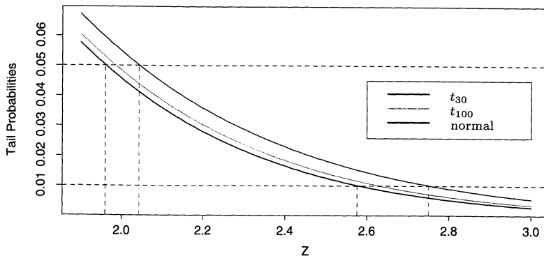
FIGURE 3.3. The tail probabilities \Pr(|Z| > z) for three distributions, t_{30} , t_{100} and standard normal. Shown are the appropriate quantiles for testing significance at the p = 0.05 and 0.01 levels. The difference between t and the standard normal becomes negligible for N bigger than about 100.
