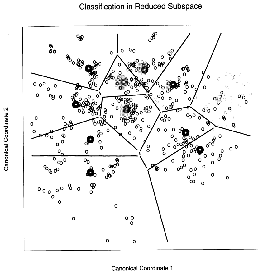
FIGURE 4.11. Decision boundaries for the vowel training data, in the two-dimensional subspace spanned by the first two canonical variates. Note that in any higher-dimensional subspace, the decision boundaries are higher-dimensional affine planes, and could not be represented as lines.
