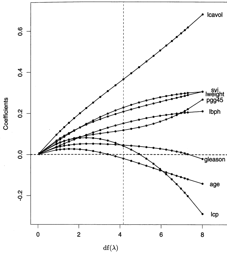
FIGURE 3.7. Profiles of ridge coefficients for the prostate cancer example, as tuning parameter \lambda is varied. Coefficients are plotted versus df(\lambda) , the effective degrees of freedom. A vertical line is drawn at df = 4.16 , the value chosen by cross-validation.
