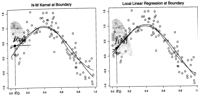
FIGURE 6.3. The locally weighted average has bias problems at or near the boundaries of the domain. The true function is approximately linear here, but most of the observations in the neighborhood have a higher mean than the target point, so despite weighting, their mean will be biased upwards. By fitting a locally weighted linear regression (right panel), this bias is removed to first order
