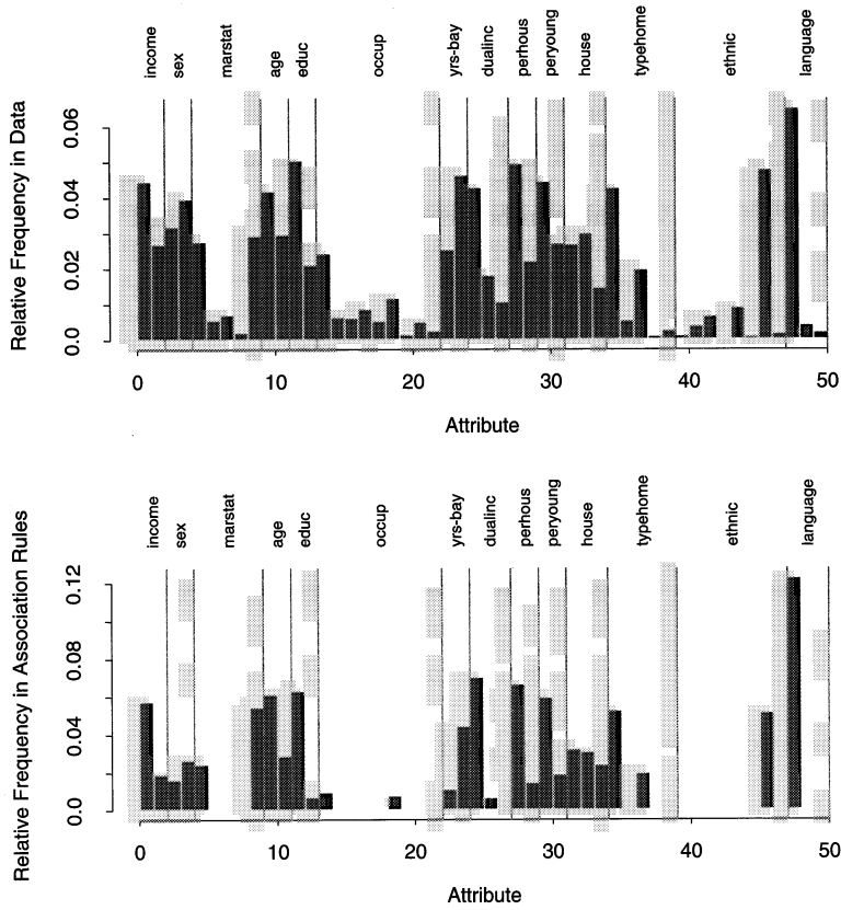
FIGURE 14.2. Market basket analysis: relative frequency of each dummy variable (coding an input category) in the data (top), and the association rules found by the Apriori algorithm (bottom).
