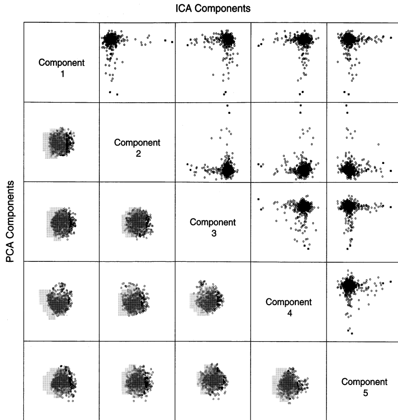
FIGURE 14.29. A comparison of the first five ICA components (above diagonal) with the first five PCA components (below diagonal). Each component is standardized to have unit variance.
