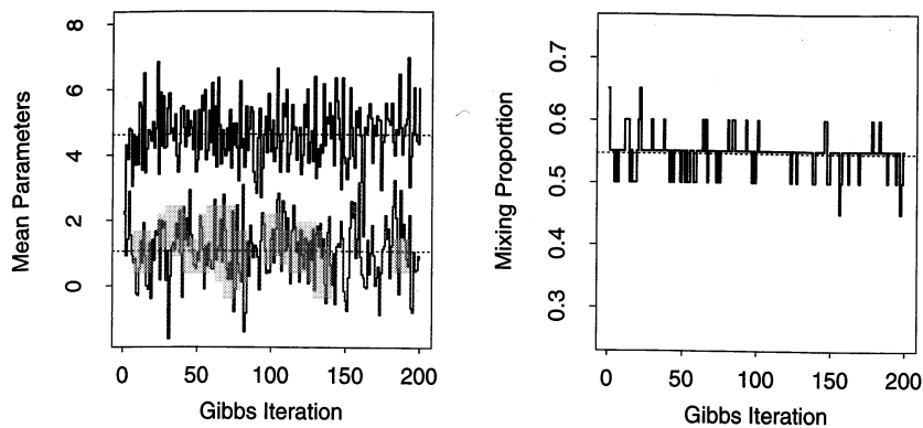
FIGURE 8.8. Mixture example. Left panel: 200 values of the two mean parameters from Gibbs sampling; horizontal lines are drawn at the maximum likelihood estimates \hat{\mu}_1 , \hat{\mu}_2 . Right panel: proportion of values with \Delta_i = 1 , for each of the 200 Gibbs sampling iterations; a horizontal line is drawn at \sum_i \hat{\gamma}_i/N .
