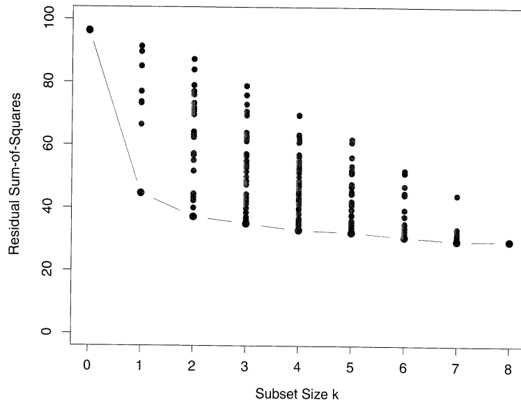
FIGURE 3.5. All possible subset models for the prostate cancer example. At each subset size is shown the residual sum-of-squares for each model of that size.
