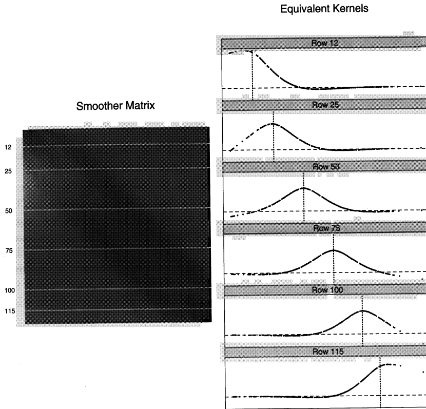
FIGURE 5.8. The smoother matrix for a smoothing spline is nearly banded, indicating an equivalent kernel with local support. The left panel represents the elements of S as an image. The right panel shows the equivalent kernel or weighting function in detail for the indicated rows.
