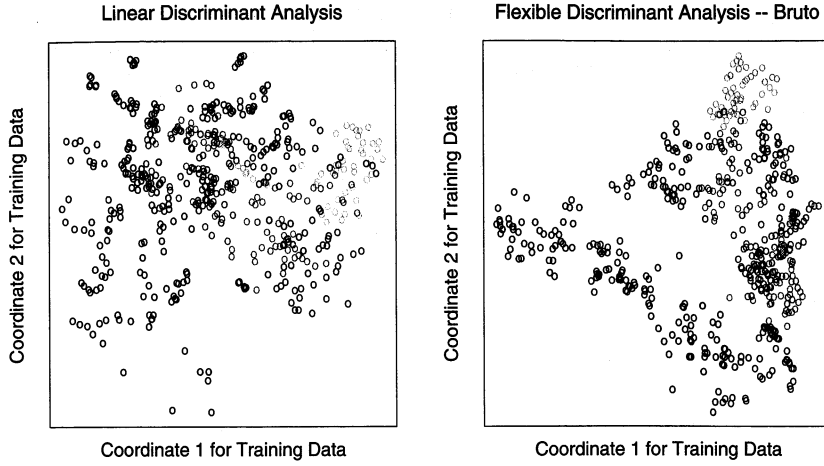
FIGURE 12.8. The left plot shows the first two LDA canonical variates for the vowel training data. The right plot shows the corresponding projection when FDA/BRUTO is used to fit the model; plotted are the fitted regression functions \hat{\eta}_1(x_i) and \hat{\eta}_2(x_i) . Notice the improved separation. The letters label the vowel sounds.
