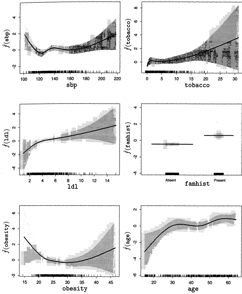
FIGURE 5.4. Fitted natural-spline functions for each of the terms in the final model selected by the stepwise procedure. Included are pointwise standard-error bands. The rug plot at the base of each figure indicates the location of each of the sample values for that variable (jittered to break ties).
