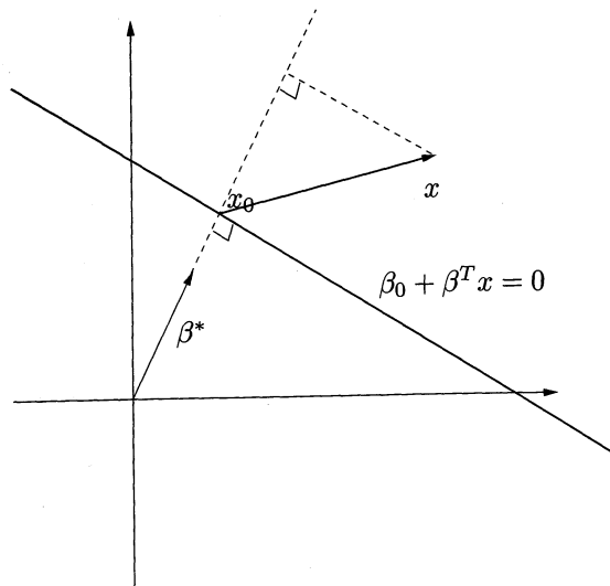
FIGURE 4.14. The linear algebra of a hyperplane (affine set).
