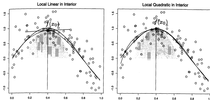
FIGURE 6.5. Local linear fits exhibit bias in regions of curvature of the true function. Local quadratic fits tend to eliminate this bias.
