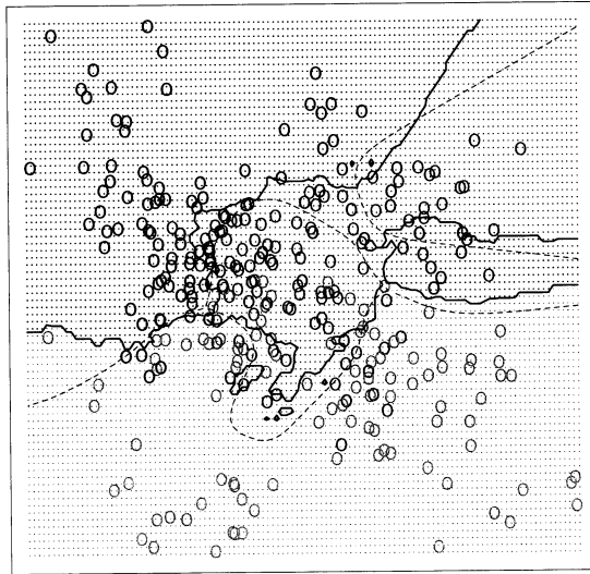
15-Nearest Neighbors
