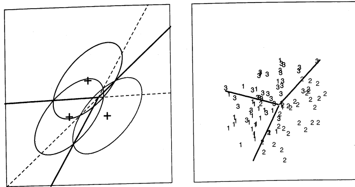
FIGURE 4.5. The left panel shows three Gaussian distributions, with the same covariance and different means. Included are the contours of constant density enclosing 95% of the probability in each case. The Bayes decision boundaries between each pair of classes are shown (broken straight lines), and the Bayes decision boundaries separating all three classes are the thicker solid lines (a subset of the former). On the right we see a sample of 30 drawn from each Gaussian distribution, and the fitted LDA decision boundaries.
