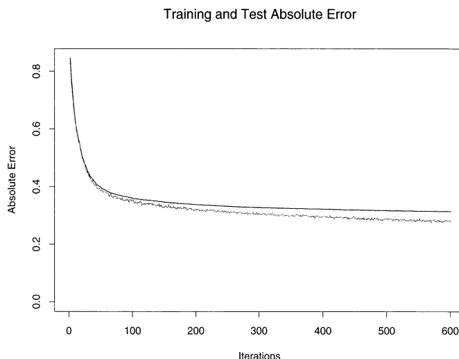
FIGURE 10.13. Average-absolute error as a function of number of iterations for the California housing data.
