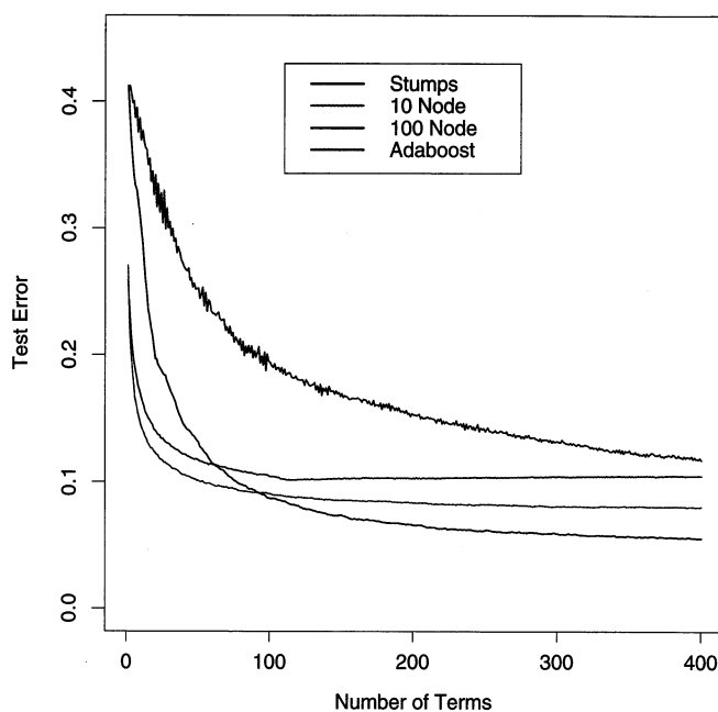
FIGURE 10.9. Boosting with different sized trees, applied to the example (10.2) used in Figure 10.2. Since the generative model is additive, stumps perform the best. The boosting algorithm used the binomial deviance loss in Algorithm 10.3; shown for comparison is the AdaBoost algorithm 10.1.
