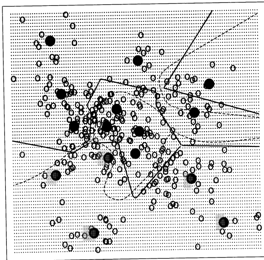
FIGURE 13.1. Simulated example with three classes and five prototypes per class. The data in each class are generated from a mixture of Gaussians. In the upper panel, the prototypes were found by applying the K-means clustering algorithm separately in each class. In the lower panel, the LVQ algorithm (starting from the K-means solution) moves the prototypes away from the decision boundary. The broken purple curve in the background is the Bayes decision boundary.
