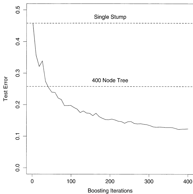
FIGURE 10.2. Simulated data (10.2): test error rate for boosting with stumps, as a function of the number of iterations. Also shown are the test error rate for a single stump, and a 400 node classification tree.
