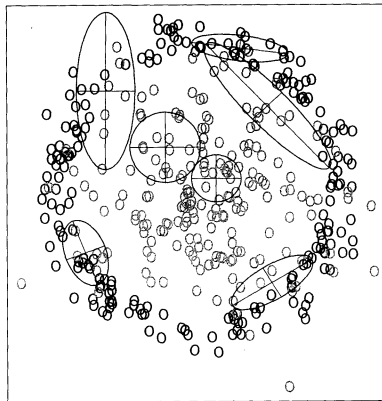
FIGURE 13.14. Neighborhoods found by the DANN procedure, at various query points (centers of the crosses). There are two classes in the data, with one class surrounding the other. 50 nearest-neighbors were used to estimate the local metrics. Shown are the resulting metrics used to form 15-nearest-neighborhoods.
