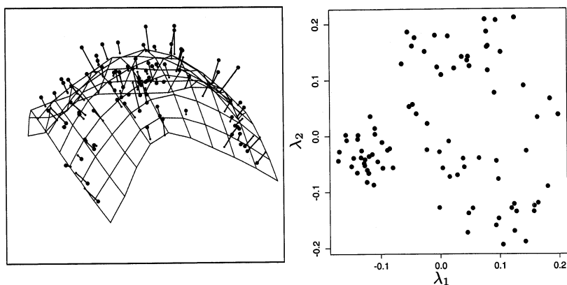
FIGURE 14.26. Principal surface fit to half-sphere data. Left panel: fitted two-dimensional surface. Right panel: projections of data points onto the surface, resulting in coordinates \lambda_1, \lambda_2 .
