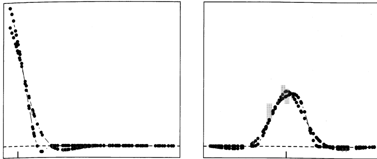
FIGURE 6.7. Equivalent kernels for a local linear regression smoother (tri-cube kernel; red) and a smoothing spline (green), with matching degrees of freedom. The vertical spikes indicates the target points.
