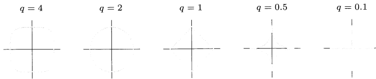
FIGURE 3.13. Contours of constant value of \sum_j |\beta_j|^q for given values of q .
