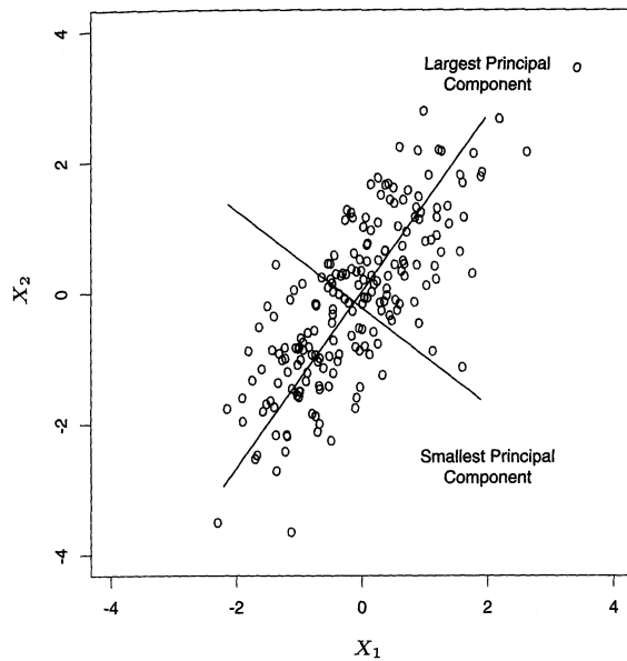
FIGURE 3.8. Principal components of some input data points. The largest principal component is the direction that maximizes the variance of the projected data, and the smallest principal component minimizes that variance. Ridge regression projects \mathbf{y} onto these components, and then shrinks the coefficients of the low-variance components more than the high-variance components.
