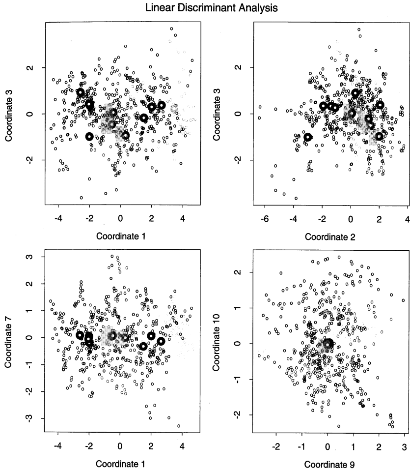
FIGURE 4.8. Four projections onto pairs of canonical variates. Notice that as the rank of the canonical variates increases, the centroids become less spread out. In the lower right panel they appear to be superimposed, and the classes most confused.
