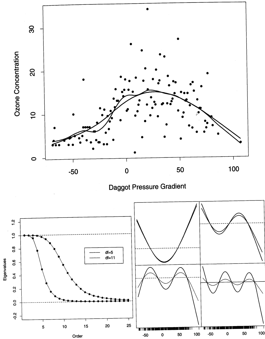
FIGURE 5.7. [Top] Smoothing spline fit of ozone concentration versus Daggot pressure gradient. The two fits correspond to different values of the smoothing parameter, chosen to achieve 5 and 11 effective degrees of freedom, defined by df_\lambda = \text{trace}(\mathbf{S}_\lambda) . [Lower left] First 25 eigenvalues for the two smoothing-spline matrices. The first two are exactly 1, and all are \geq 0 . [Lower right] third to sixth eigenvectors of the spline smoother matrices. In each case, \mathbf{u}_k is plotted against \mathbf{x} , and as such is viewed as a function of x . The rug at the base of the plots indicate the occurrence of data points. The damped functions represent the smoothed versions of these functions (using the 5df smoother).
