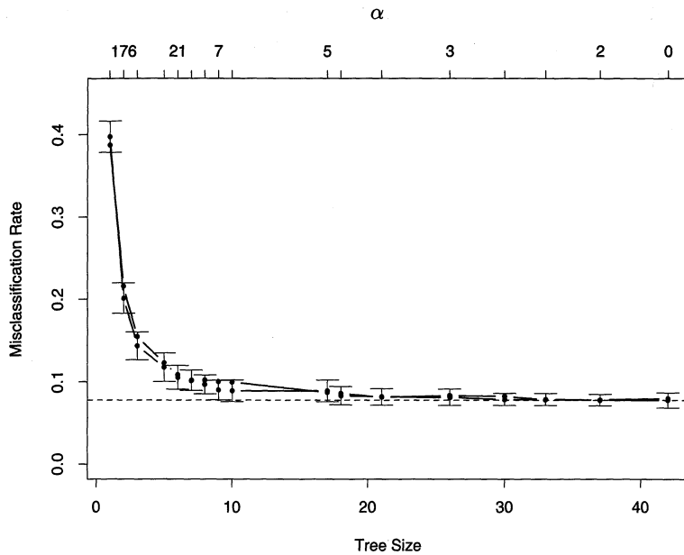
FIGURE 9.4. Results for spam example. The green curve is the tenfold cross-validation estimate of misclassification rate as a function of tree size, with \pm two standard error bars. The minimum occurs at a tree size with about 17 terminal nodes. The red curve is the test error, which tracks the CV error quite closely. The cross-validation was indexed by values of \alpha , shown above. The tree sizes shown below refer to |T_\alpha| , the size of the original tree indexed by \alpha .
